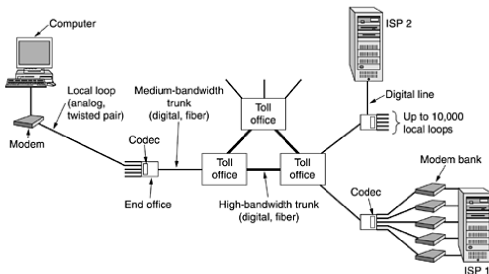
Figure 2-23. The use of both analog and digital transmission for a computer to computer call. Conversion is done by the modems and codecs.
