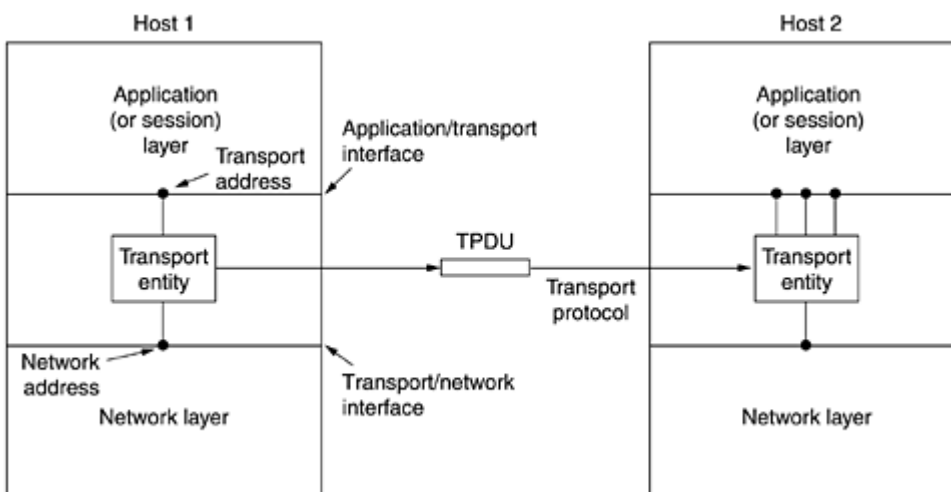
Figure 6-1. The network, transport, and application layers.
